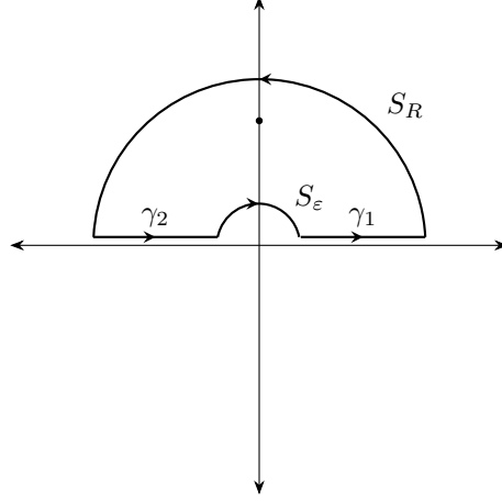
Figure 10: The contour \Gamma_{R,\varepsilon} with a pole of f at ai .
